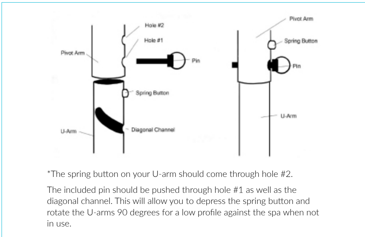
Figure 2 - Attaching U-arms to pivot arm (Step 5)
